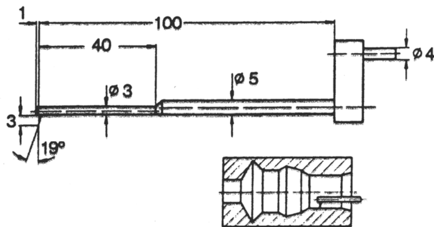
(c) 小孔用支臂
